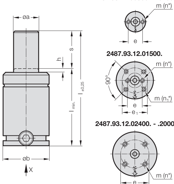
View/Design X - gas spring 2487.93.12.00350. - .01000. .1
