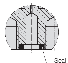
View/Design gas spring with flat seal
