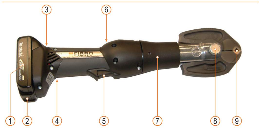
Fig. 3-1 Structure
