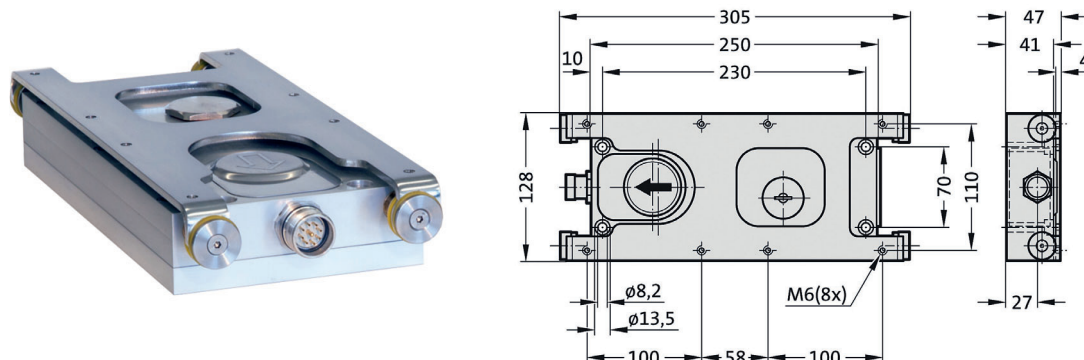
Fig. 3-3 Dimensions of electric transporter CLEAN LINE COMPACT
