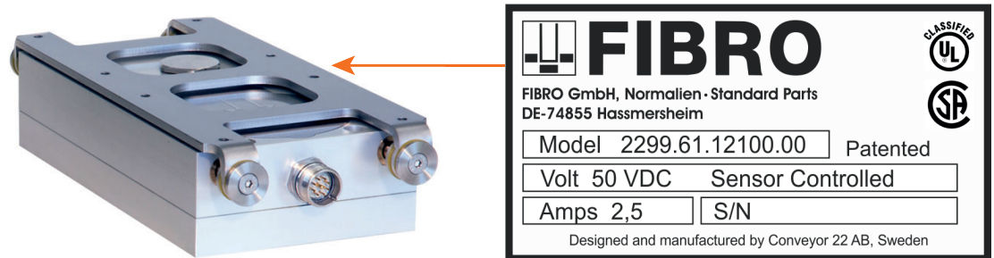
Fig. 3-5 Type plate
