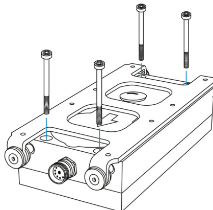
Fig. 5-4 Mounting electric transporter
